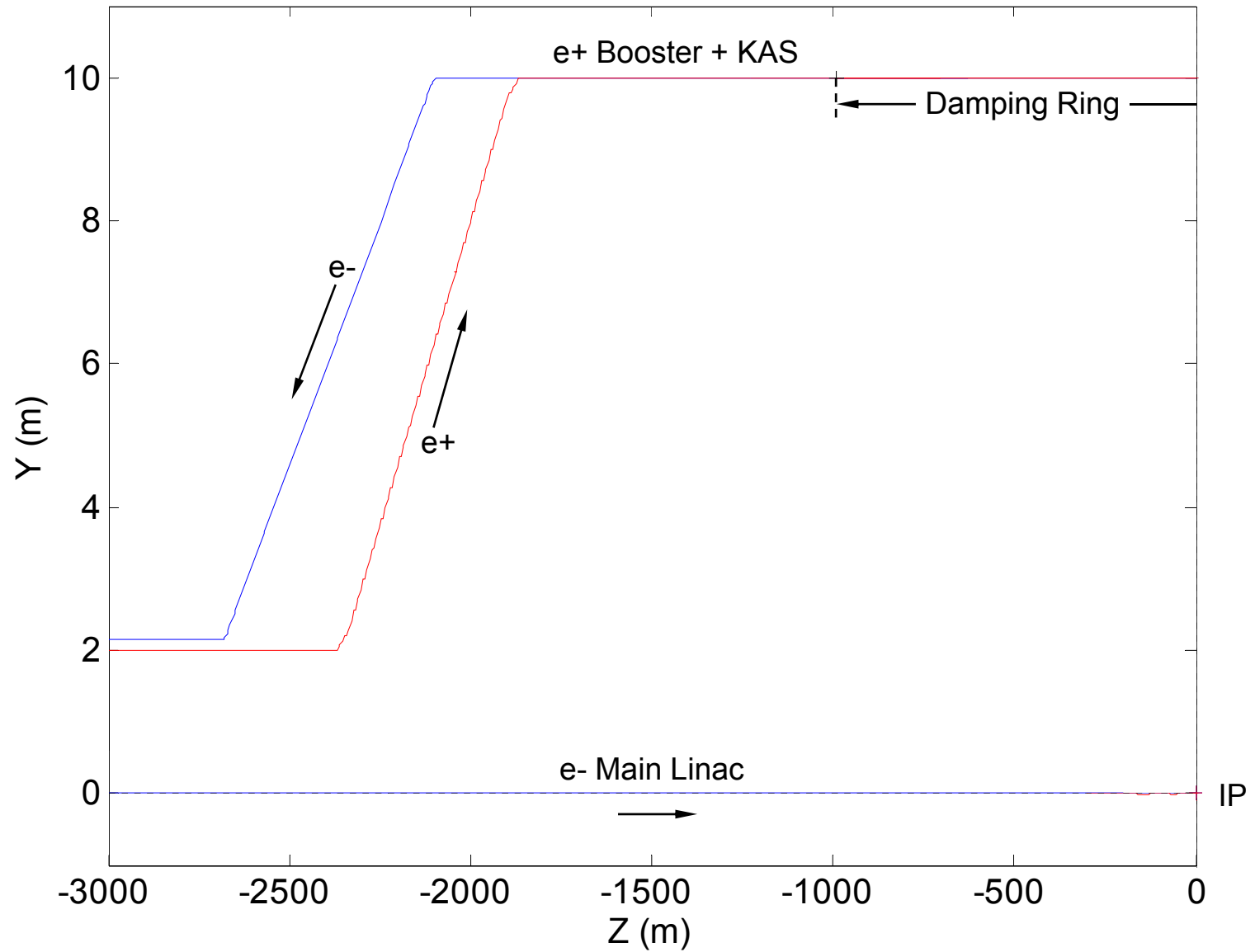
Elevation View (anamorphic scale)
