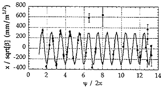
Fig. 2 The fit of a leakage orbit to a sinusoidal curve. The ordinate is the orbit normalized by \beta^{1/2} and the abscissa is the phase advance from ST1 (divided by 2\pi ). The error bars represent the statistical noise in the orbit measurement.
