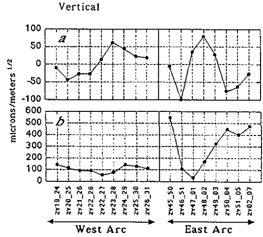
Fig. 3 The observed coefficients a and b of leakage orbits for the vertical bumps in West and East Arc. The bumps are named by the correctors to produce it.
