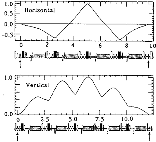
Fig. 1 Geometrical shape of a horizontal (upper figure) and a vertical (lower) bump orbit in the arc. The orbits are normalized by their maximum values. The abscissas are s (meters). The lattice configurations are shown in the bottom of each picture. The correctors to excite the bump are pointed by arrows. The magnets of QF2R (quadrupole, horizontally focusing) in the bump region are painted out and those of BH1R (combined bend, horizontally defocusing) are shaded in the figure.
