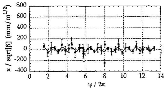
Fig. 5 Observed leakage orbit after correction. Compare this orbit with the orbit before correction, shown in Fig. 2. In this example, the target was QF2R.25. The elimination of b component of the leakage orbit indicates the phase is tuned to be its design value ( 3\pi ). We find a = -11 \pm 18 and b = -38 \pm 18(\text{microns/meters}^{1/2}) .
