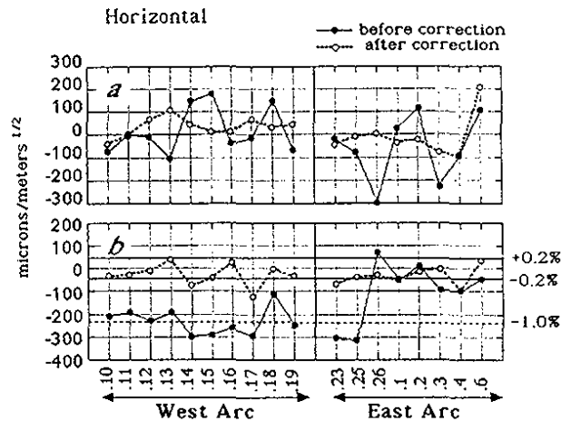
Fig. 6 The coefficients a and b of the fit for the horizontal leakage orbits of the first (before correction) and the second (after correction) measurement. The bumps are named by the target magnets. The strength of the targets was changed by the data fitted b of the first measurement. If the target deviates 0.2%, it produces b component leakage orbit of 50 microns/meter 1/2 . This and the level of 1% target error are shown as the horizontal line in the bottom figure.
