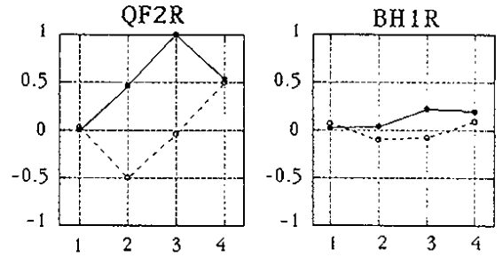
Fig. 4 Values of W_a (dotted line) and W_b (solid line) at QF2R and BH1R magnets in the horizontal \pi -bump. The magnets are numbered from upstream to downstream. The values of W_a and W_b are normalized by the W_b at the third QF2R magnet. This magnet, which locates almost the center of the bump region, has the maximum weight in the summation for b .
