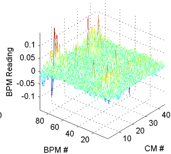
Measured Response Matrix (VBPM-HCM) Measured-Model Response Matrix (VBPM-HCM)
