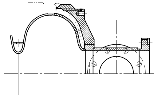
STF 1.5(35MV/m) (Front View)
