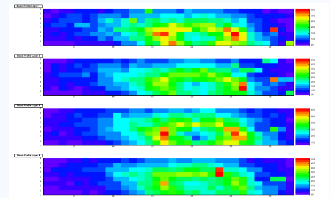
Beam profile
