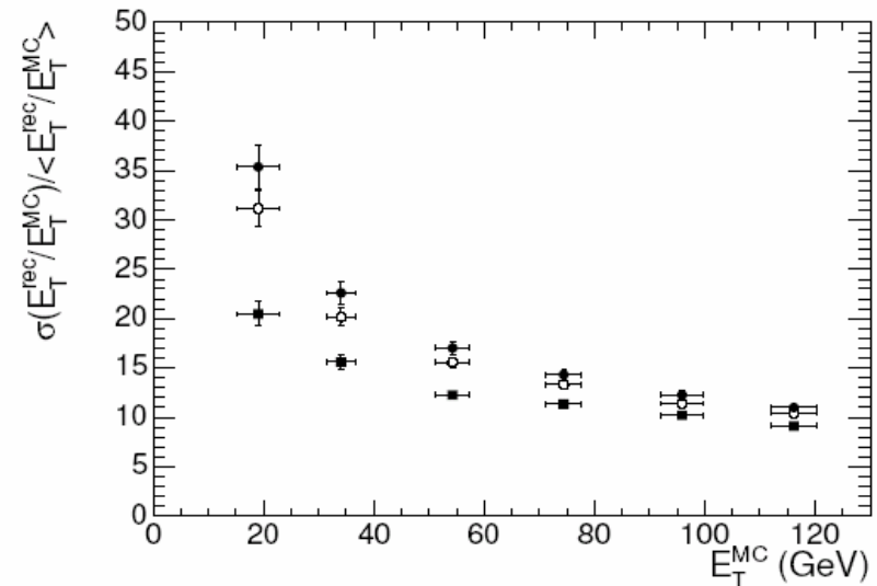
Cone 0.5 - \eta < 0.3
