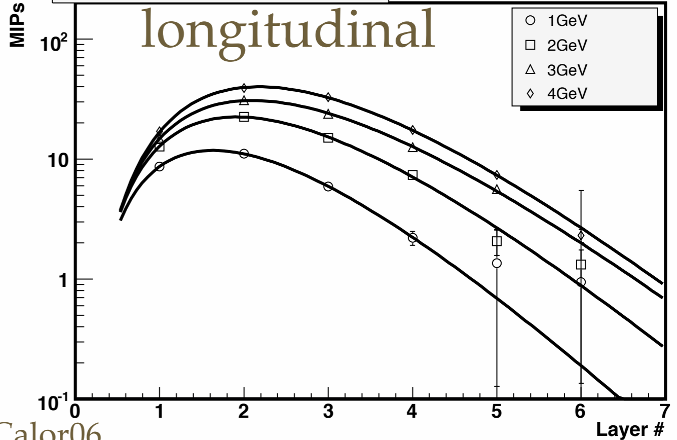
Shower Curve 1GeV to 4GeV
