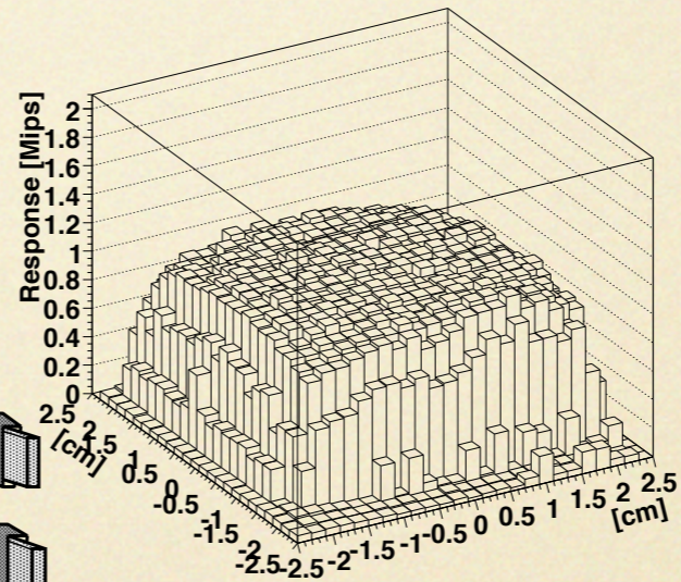
Shower Curve 1GeV to 4GeV
