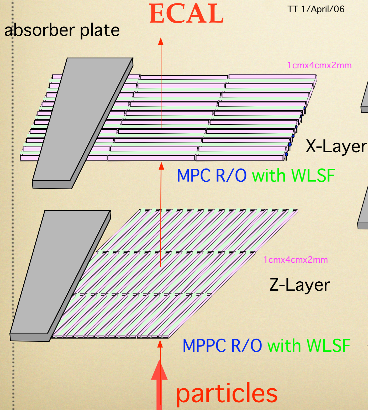
GLD-ECAL-Scintillator-layer model
