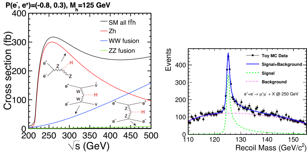
Figure 8.1: Left: Cross sections for the three major Higgs production processes as a function of center of mass energy [2]. The Zh “Higgs-strahlung” process dominates at 250 GeV. Right: Recoil mass spectrum against Z \rightarrow \mu^+\mu^- for signal e^+e^- \rightarrow Zh and SM background at 250 GeV [163].
