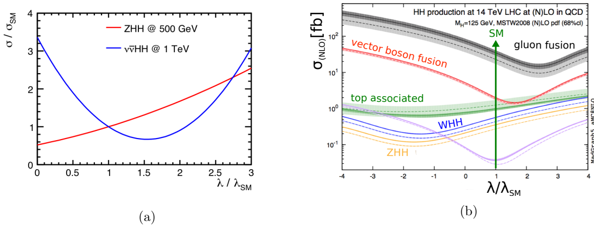
Figure 10.3: (a) Cross-sections for double Higgs production via Higgs-strahlung (at \sqrt{s} = 500 GeV) and WW fusion (at 1 TeV) as a function of the triple-Higgs coupling (normalised to its SM value) [247]. (b) Analogous graphs for double-Higgs production modes at the LHC [248]. Fusion-type processes exhibit qualitatively the same behaviour in pp as in e^+e^- collisions, and the same similarity between pp and e^+e^- can be observed for the strahlungs-like processes. Note that at LHC, double-Higgs-strahlung is burried by many orders of magnitude below fusion-type processes.
