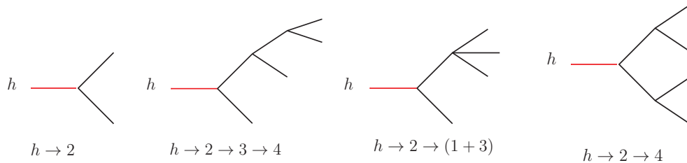
Figure 8.3: Representative topologies of the Higgs exotic decays.
