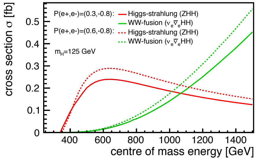
Figure 10.2: Cross-sections for double Higgs production via Higgs-strahlung and WW fusion as a function of the center-of-mass energy [247].
