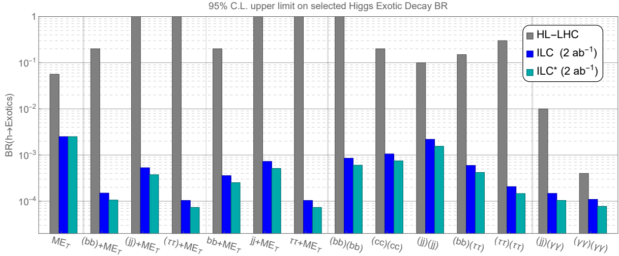
Figure 8.5: The 95% C.L. upper limit on selected Higgs exotic decay branching fractions at HL-LHC and ILC, based on Ref [174]. The ILC curves are derived using results from Ref [174] with leptonic decaying Z boson in the e^-e^+ \rightarrow ZH process. The ILC* scenario further utilizes the hadronically decaying Z boson and includes an estimated (indicative) improvement of 40%. We put several vertical lines in this figure to divide different types of Higgs exotic decays.
