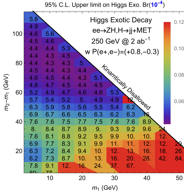
Figure 8.4: The 95% C.L. upper limit on the Higgs exotic decay branching fractions into jj + \cancel{E}_T for various lightest detector-stable particle mass m_1 and mass splittings m_2 - m_1 .
