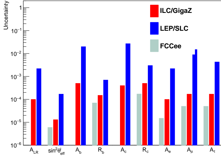
Figure 9.1: Summary of the precision achievable for ILC Z-Pole running compared with LEP/SLC results [269] and FCCee projections [?] for observables and derived quantities that are described in the text.
