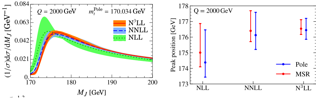
Figure 8.12: (a) The jet mass distribution on boosted top quark jets. (b) The peak position extracted using Pole mass or MSR mass schemes.
