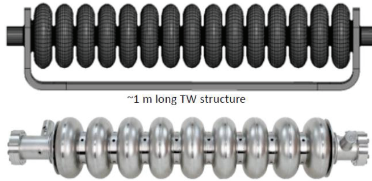
Figure 4.23: The TW structure compared to the one-meter standing-wave ILC structure.
