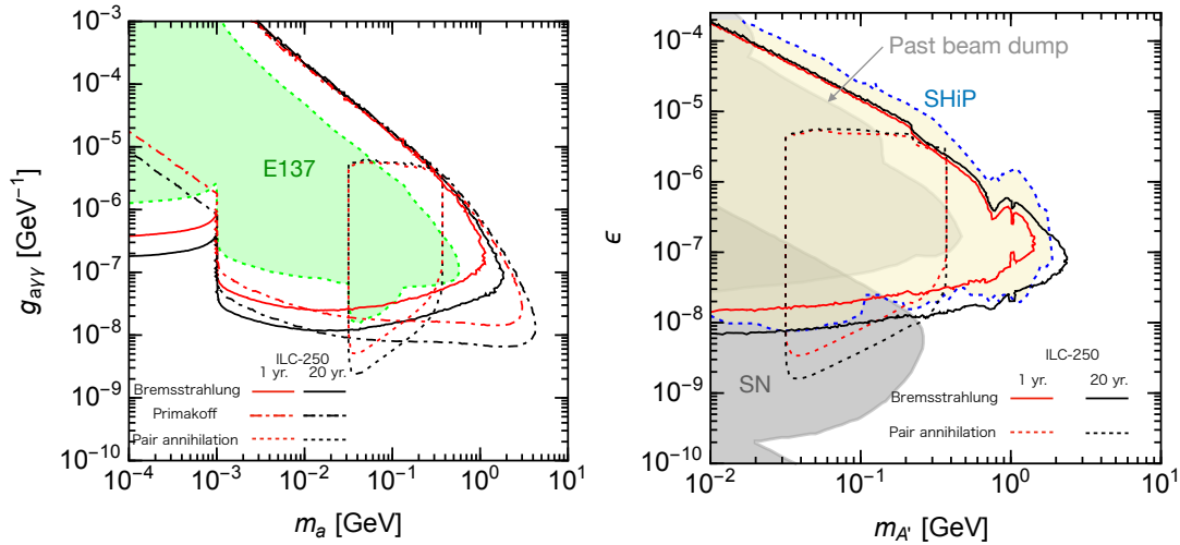
Figure 11.2: The reach of a beam-dump experiment at the ILC-250 for axion-like particles (left) and dark photons (right). Taken from Ref. [396]. See also [397] for another study of the reach on axion-like particles.
