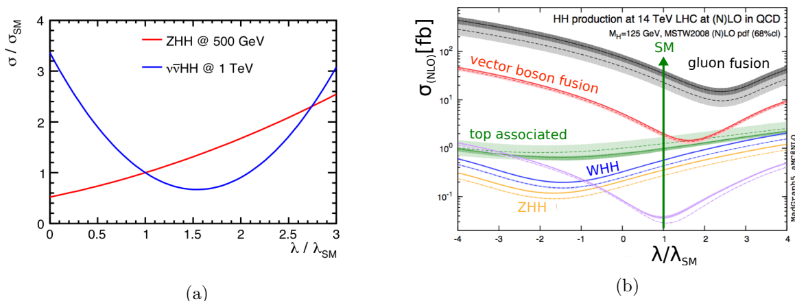
Figure 10.4: (a) Cross-sections for double Higgs production via Higgs-strahlung (at \sqrt{s} = 500 \text{ GeV} ) and WW fusion (at 1 \text{ TeV} ) as a function of the triple-Higgs coupling (normalised to its SM value) [325]. (b) Analogous graphs for double-Higgs production modes at the LHC [326]. Fusion-type processes exhibit qualitatively the same behaviour in pp as in e^+e^- collisions, and the same similarity between pp and e^+e^- can be observed for the Higgs-strahlungs-like processes. Note that at LHC, double-Higgs-strahlung is buried by many orders of magnitude below fusion-type processes.
