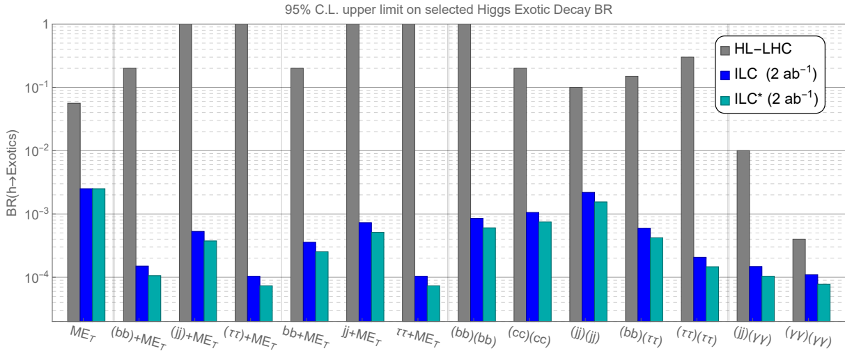
Figure 8.6: The 95% C.L. upper limit on selected Higgs exotic decay branching fractions at HL-LHC and ILC, based on Ref [235]. The ILC curves are derived using results from Ref [235] with leptonic decaying Z boson in the e^-e^+ \rightarrow ZH process. The ILC* scenario further utilizes the hadronically decaying Z boson and includes an estimated (indicative) improvement of 40%. Each set of three bars describes a different topology of exotic Higgs decay.
