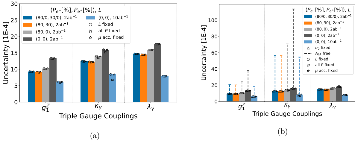
Figure 8.7: (a) Expected precisions at \sqrt{s} = 250 GeV on charged TGCs for different assumptions on the beam polarizations and the integrated luminosity. Note that these appear more pessimistic than in Fig. 10.6 since here only the \mu\nu qq channel is used in a binned three-angle analysis (b) Effect of floating the left-right asymmetry of the the Zee coupling in the fit. This underlines, first, the importance of independently measuring this this quantity — not only on the Z pole, but at 250 GeV — and, second, the increased robustness of the fit due to beam polarization, which reduces the dependence on the left-right asymmetry considerably. Both from [268, 269].
