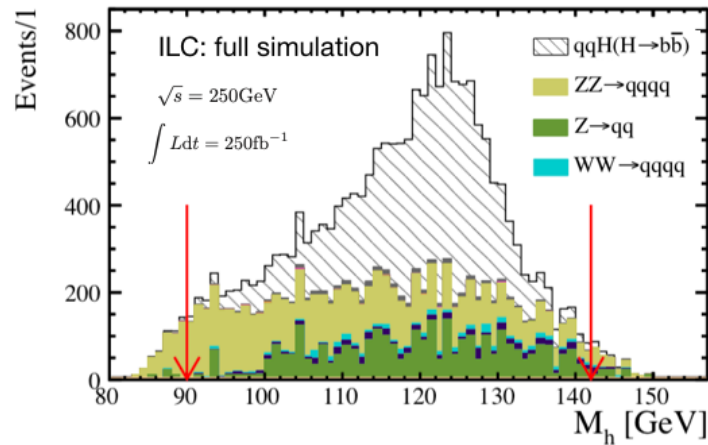
Figure 8.3: Comparison of signal and backgrounds from ILD full simulation for the measurement of \sigma \times BR for H \rightarrow b\bar{b} , for 250 \text{ fb}^{-1} of ILC data at 250 GeV, from [226].
