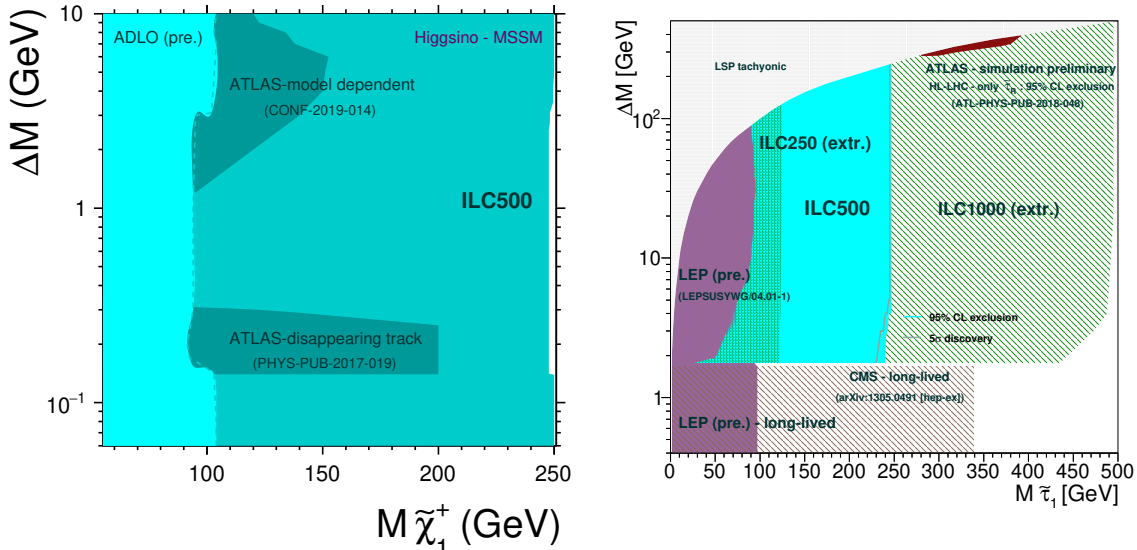
Figure 10.7: Exclusion and discovery reaches for a \tilde{\chi}_1^\pm (left), or a \tilde{\tau}_1 (right).
