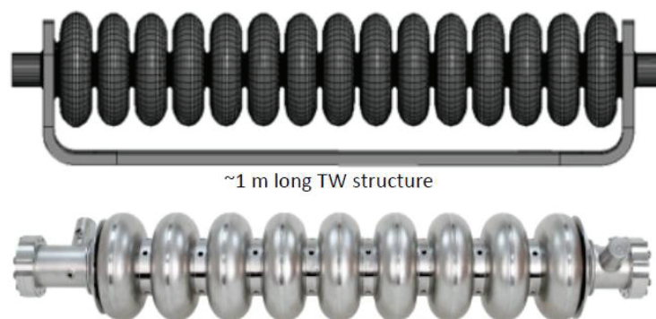
Figure 4.29: The TW structure compared to the one-meter standing-wave ILC structure.
