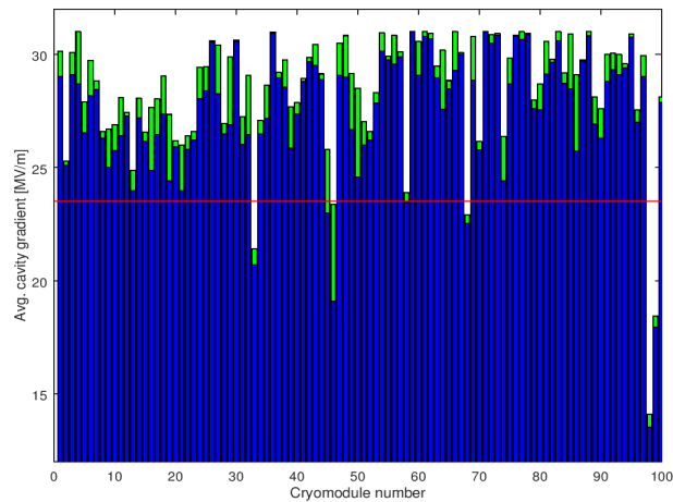
Figure 4.8: Average of the operating (blue) and maximum (green) gradient for cavities in each European XFEL serial-production cryomodule. The specification of 23.6 MV/m is marked by a red line [60]. Modules 98 and 99 were assembled from the lowest-performing cavities.
