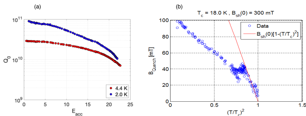
Figure 4.31: (a) Record CW behavior for Nb 3 Sn coated with solid state diffusion method at Fermilab showed E_{acc} = 23 MV/m. Excellent performance was obtained by making a smooth thin film about 1 \mu\text{m} . (b) Measurements of the critical RF field of Nb 3 Sn using high power pulsed RF. The high temperature results extrapolate to a maximum surface magnetic field of 300 mT, which would translate to E_{acc} = 85 MV/m for a Low-Loss shape cavity.
