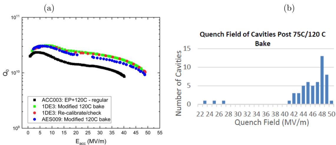
Figure 4.27: (a): Q vs. E curve of 1-cell cavity reaching 49 MV/m from Cold EP/optimized baking (75/120 C) compared to the curve of a cavity prepared by the standard ILC recipe. (b) Histogram of gradients of a large number of single cell cavities prepared by Cold EP/optimized baking (75/120 C).
