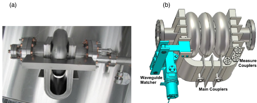
Figure 4.30: (a) 1-cell TW Niobium structure with return waveguide, treated by BCP and tested to reach 26 MV/m. (b) 3-cell TW structure built but not yet tested.
