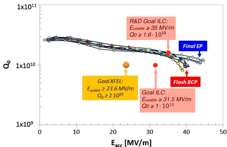
Figure 4.4: Examples of the Q_0(E_{acc}) curves of some of the best cavities, either treated at RI using “EP final”, or at EZ using “BCP flash.” [48, Fig. 19]. Vendor “RI” employs a production process that closely follows the ILC specifications, with a final electropolishing step. The ILC gradient / Q_0 goals are overlaid.
