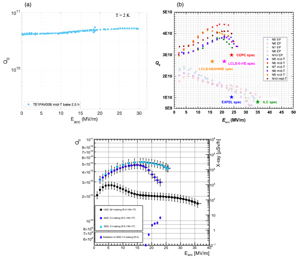
Figure 4.25: (a) Q = 5 \times 10^{10} at 30 MV/m by baking at 300 C to dissolve the natural oxide (and other surface layers) into the bulk, but not exposing the cavity to air or water before RF measurements; (b) IHEP (China) results on mid-T baking for 9-cell cavities compared to results on the same cavities with the standard ILC treatment [132]; (c) 300 C baking results from KEK on single cell cavities after high pressure water rinsing. Standard ILC treatment results are also included.
