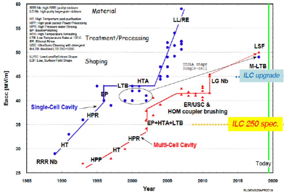
Figure 4.23: Steady progress in single and multi-cell cavity gradients over 3+ decades [126].
