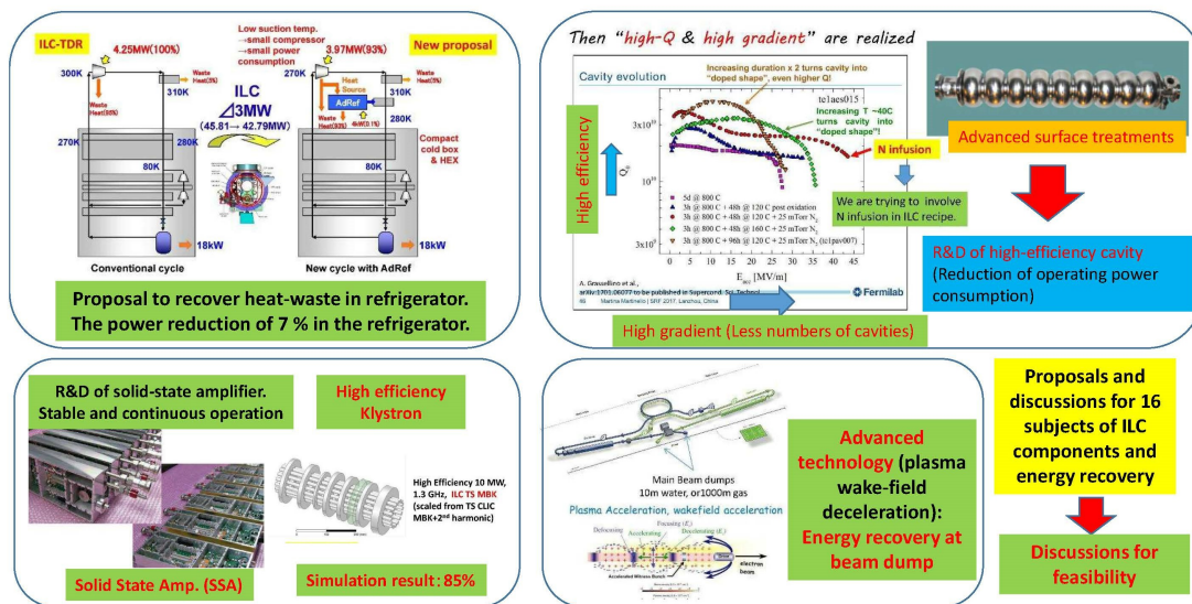
Figure 4.18: R&D of high-efficiency components of ILC. Upper left: a proposal for efficient refrigerator, lower left: proposals of high efficiency power source, upper right: examples of high-Q and high-gradient cavities, lower right: a proposal of beam dump with wake field deceleration.
