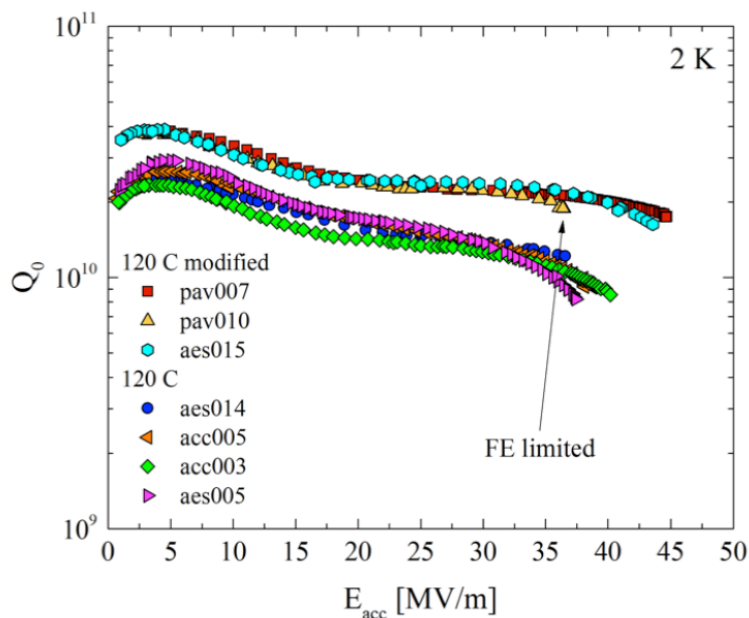
Figure 4.26: Comparison of the performance of several 1-cell cavities from N-infusion with cavities prepared by the standard ILC recipe of EP and 120 C baking.
