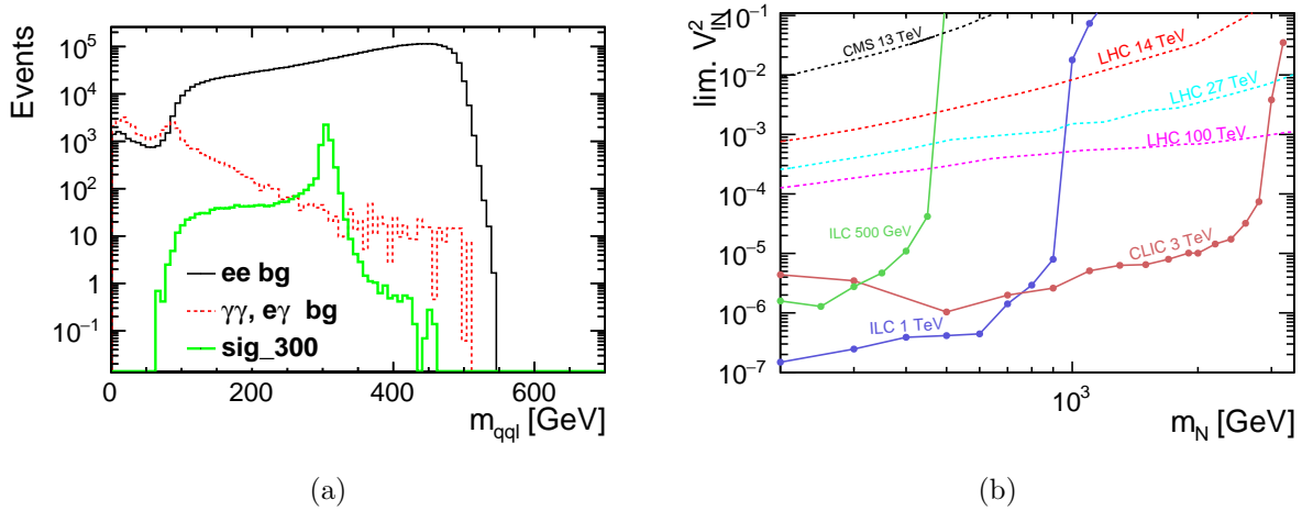
Figure 10.19: Left: qq l mass distribution for ILC500 for muons in the final state. Black solid line stands for the e^+e^- background, red dashed line for the \gamma -induced background and thick green line for a reference signal scenario (Dirac neutrino with a mass of 300 GeV). Right: limits on the coupling V_{IN}^2 for different colliders (solid lines: ILC500 – green, ILC1000 – violet, CLIC3000 – dark red). Dashed lines indicate limits from current and future hadron colliders based on [560, 561]. Figure taken from [562].
