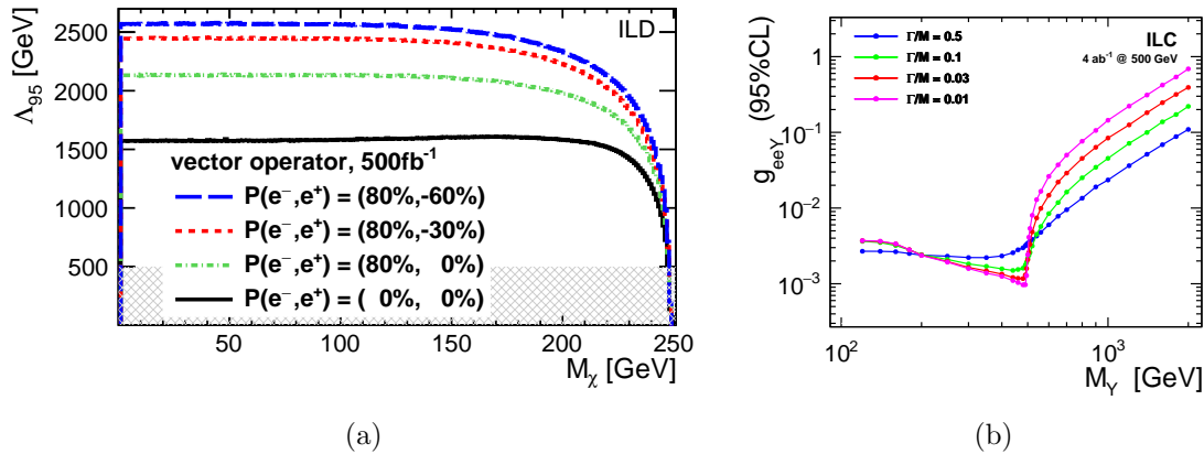
Figure 10.16: (a): Observational reach ( 2\sigma ) of the ILC for a fermionic WIMP with a WIMP-fermion vector coupling in terms of the WIMP mass for four different beam-polarization configurations [539]. (b): Expected limits on the vector mediator coupling to electrons for the ILC running at 500 GeV and different fractional mediator widths, as a function of the mediator mass [540].
