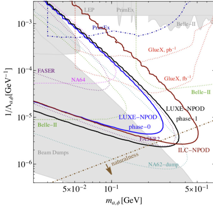
Figure 11.4: Sensitivity of the ILC version of the LUXE-NPOD experiment [576] searching for scalar and axion-like particles that couples to photons. The sensitivity is expressed in terms of parameters \Lambda_a and \Lambda_\phi defined in eq. (11.1).
