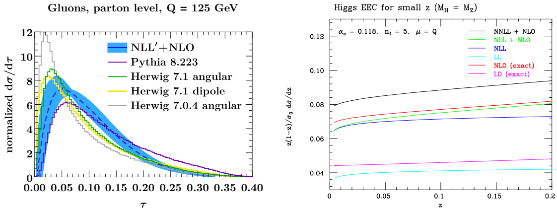
Figure 8.11: Precision perturbative calculations in H \rightarrow gg . In (a) we show a double logarithmic Sudakov event shape observable [372], and in (b) and single logarithmic collinear observable [370].
