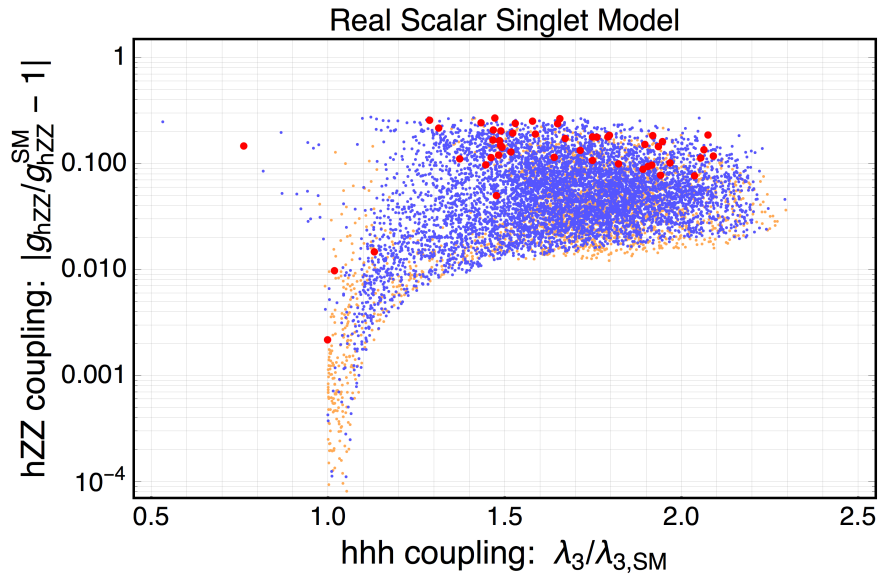
Figure 13.2: Scan of the parameter space for a model of baryogenesis at the electroweak scale with one new electroweak singlet Higgs field mixing with the SM Higgs doublet, from [605]. Blue points represent models with a strong first-order electroweak phase transition, required for successful baryogenesis.
