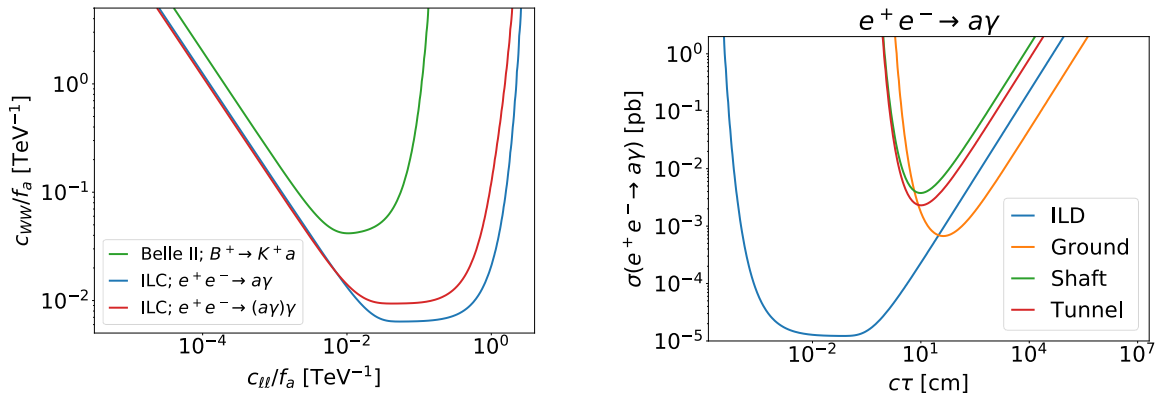
Figure 10.23: Left panel: Sensitivity projections for long-lived ALPs with m_a = 300 MeV at the ILC and at Belle II, as a function of the couplings c_{WW}/f_a and c_{ll}/f_a . Right panel: Sensitivity projections for long-lived ALPs with m_a = 300 MeV at the ILC main detector (ILD), and three dedicated far-detector options (Ground, Shaft, and Tunnel). From Ref. [570].
