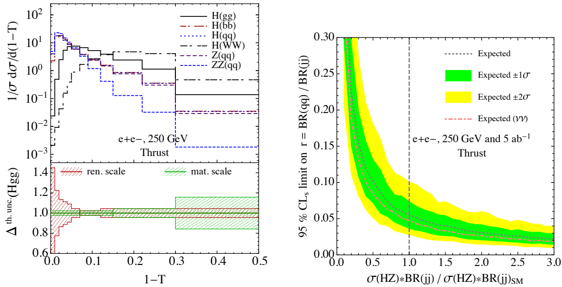
Figure 8.12: Precision measurements of event shapes on Higgs decays used to bound the light quark Yukawas [373].
