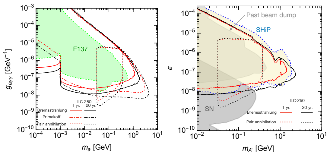
Figure 11.2: The reach of a beam-dump experiment at the ILC-250 for axion-like particles (left) and dark photons (right). Taken from Ref. [573]. See also [574] for another study of the reach on axion-like particles.
