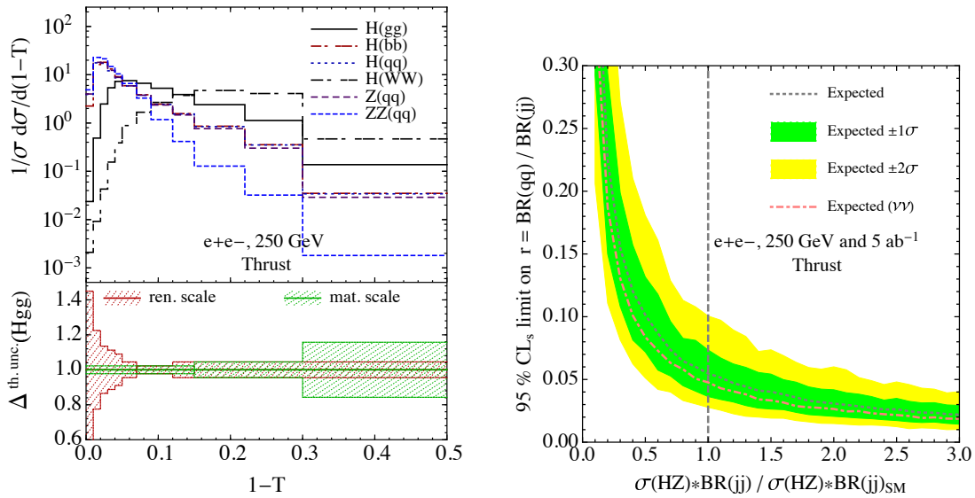
Figure 8.12: Precision measurements of event shapes on Higgs decays used to bound the light quark Yukawas [374].
