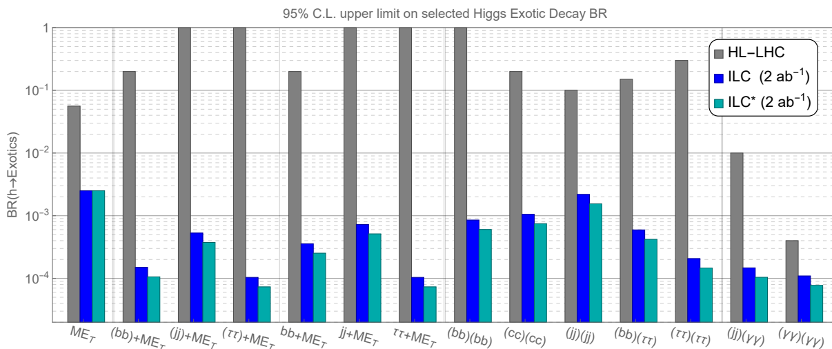
Figure 8.7: The 95% C.L. upper limit on selected Higgs exotic decay branching fractions at HL-LHC and ILC, based on Ref [318]. The ILC curves are derived using results from Ref [318] with leptonic decaying Z boson in the e^-e^+ \rightarrow ZH process. The ILC* scenario further utilizes the hadronically decaying Z boson and includes an estimated (indicative) improvement of 40%. Each set of three bars describes a different topology of exotic Higgs decay. For a recent review on current LHC constraints, see Ref. [320].
