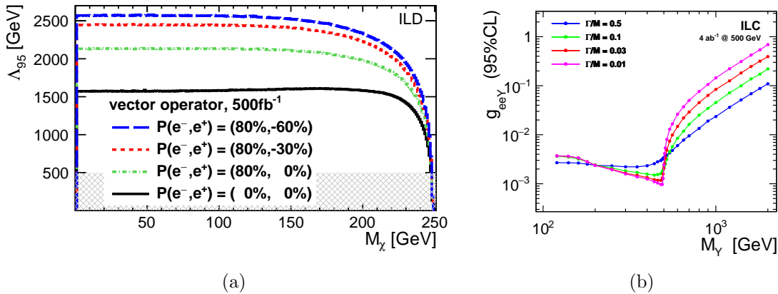
Figure 10.16: (a): Observational reach ( 2\sigma ) of the ILC for a fermionic WIMP with a WIMP-fermion vector coupling in terms of the WIMP mass for four different beam-polarization configurations [546]. (b): Expected limits on the vector mediator coupling to electrons for the ILC running at 500 GeV and different fractional mediator widths, as a function of the mediator mass [547].
