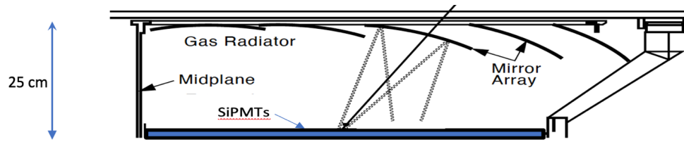
Figure 6.16: Proposed gaseous RICH detector addition to SiD/ILD [276].
