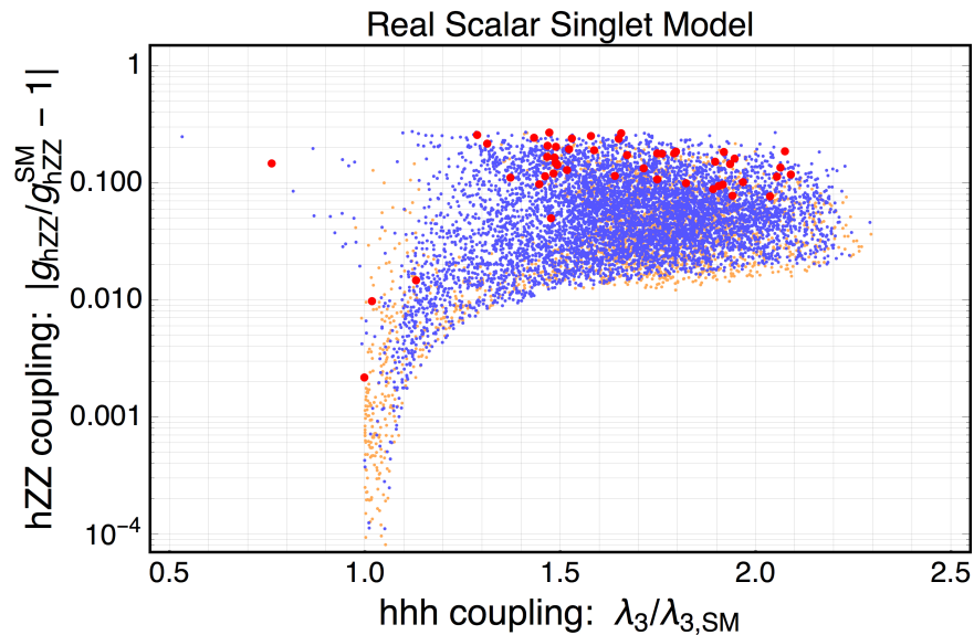
Figure 13.2: Scan of the parameter space for a model of baryogenesis at the electroweak scale with one new electroweak singlet Higgs field mixing with the SM Higgs doublet, from [616]. Blue points represent models with a strong first-order electroweak phase transition, required for successful baryogenesis.
