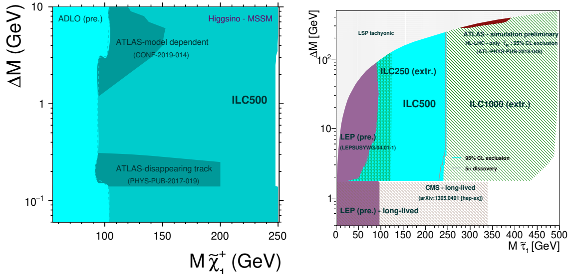
Figure 10.11: Exclusion and discovery reaches for a \tilde{\chi}_1^\pm (left), or a \tilde{\tau}_1 (right). In both cases, the horizontal axis is the mass of the charged SUSY particle and the vertical axis is the mass splitting between this state and the (neutral) lightest SUSY particle.
