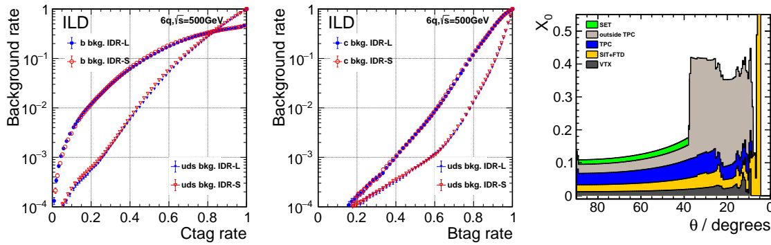
Figure 6.2: Flavour tag performance for the large and small ILC detector models. Background rate as a function of the c-tagging (left) and b-tagging (middle) efficiency for heavy quark and light flavour quark jets. Right: Material budget in ILC up to the calorimeter, in fraction of a radiation length. The different contributions are summed up to represent the cumulative radiation length at a given polar angle. (Figures from [213])
