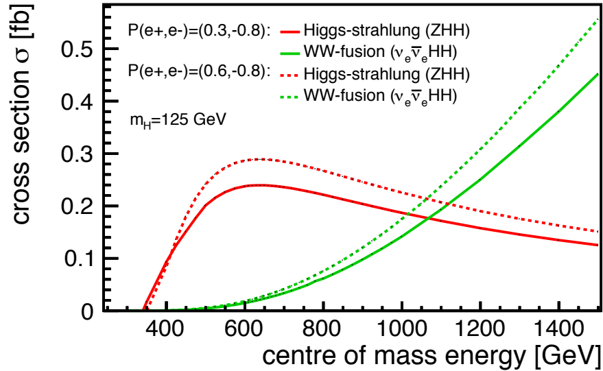
Figure 10.6: Cross-sections for double Higgs production in the SM via Higgs-strahlung and WW fusion as a function of the center-of-mass energy [510].
