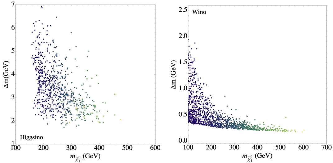
Figure 14.1: Scans over the parameter set of the MSSM giving models that account for the current discrepancy between the observed value of the muon g - 2 and the consensus SM prediction, from [675]. Left: Higgsino LSP; Right: Wino LSP. Other scenarios are described in the text. Color encodes the predicted value of the LSP dark matter density, with green indicating a higher value.
