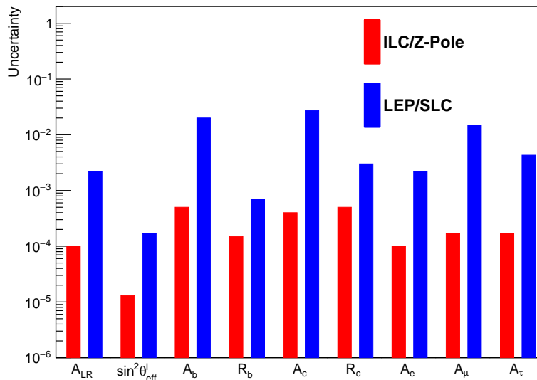
Figure 9.3: Summary of the precision achievable for ILC Z-Pole running compared with LEP/SLC results [425] for observables and derived quantities that are described in the text.
