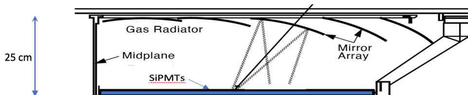
Figure 6.16: Proposed gaseous RICH detector addition to SiD/ILD [299].
