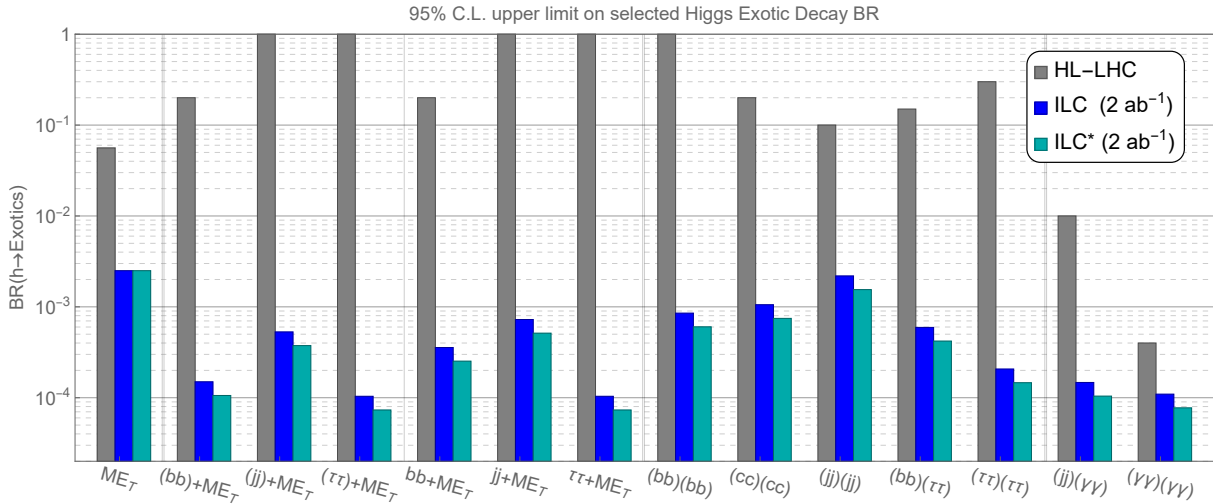
Figure 8.7: The 95% C.L. upper limit on selected Higgs exotic decay branching fractions at HL-LHC and ILC, based on Ref [345]. The ILC curves are derived using results from Ref [345] with leptonic decaying Z boson in the e^-e^+ \rightarrow ZH process. The ILC* scenario further utilizes the hadronically decaying Z boson and includes an estimated (indicative) improvement of 40%. Each set of three bars describes a different topology of exotic Higgs decay. For a recent review on current LHC constraints, see Ref. [347].
