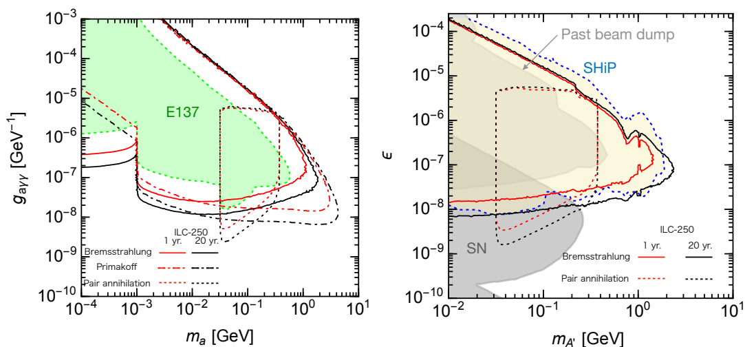
Figure 11.2: The reach of a beam-dump experiment at the ILC-250 for axion-like particles (left) and dark photons (right). Taken from Ref. [625]. See also [626] for another study of the reach on axion-like particles.
