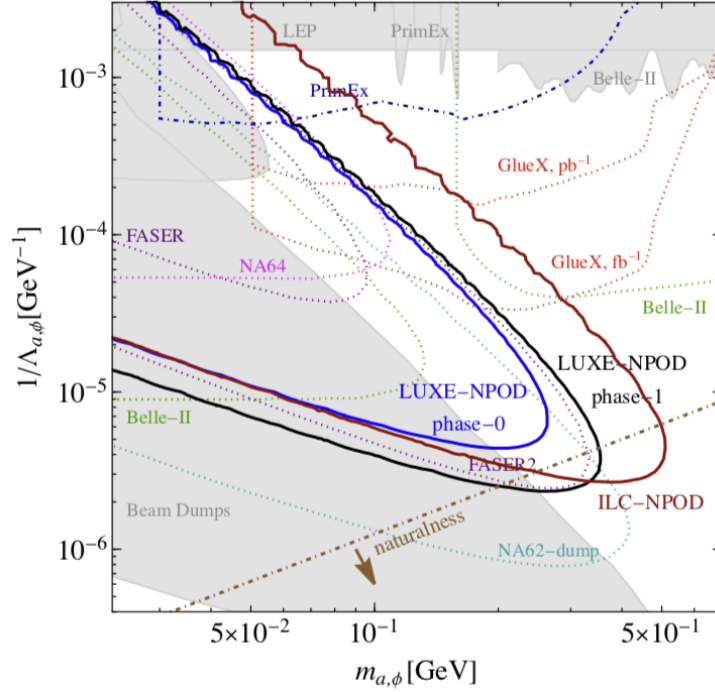
Figure 11.4: Sensitivity of the ILC version of the LUXE-NPOD experiment [630] searching for scalar and axion-like particles that couples to photons. The sensitivity is expressed in terms of parameters \Lambda_a and \Lambda_\phi defined in eq. (11.1).
