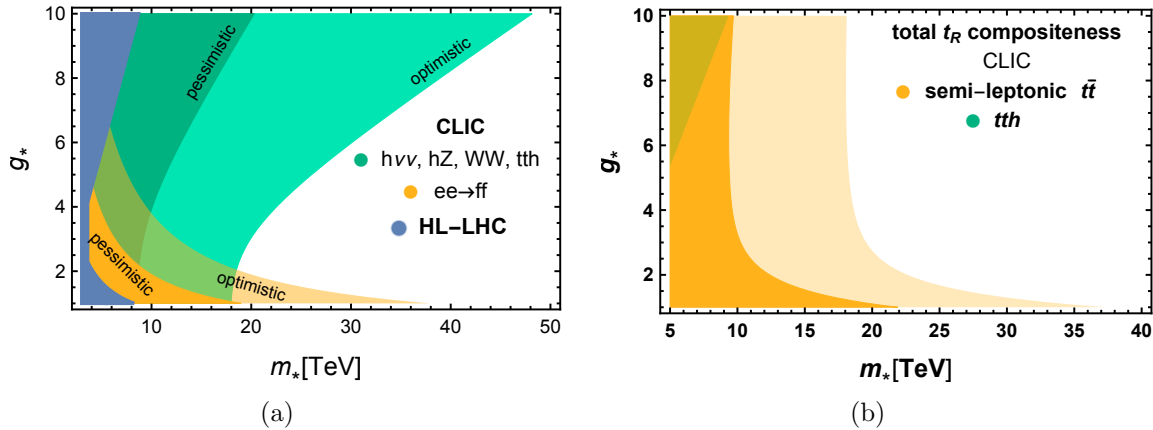
Figure 15.2: Composite Higgs reach from Higgs boson, top quark and Drell-Yan studies taken from Refs. [507] and [478]. Left panel: 5\sigma discovery contours for Higgs compositeness in the (m_*, g_*) plane, and as well the 2\sigma projected exclusions from the HL-LHC. Right panel: The 5\sigma top quark compositeness discovery contours in the (m_*, g_*) planes from studies of t\bar{t} and t\bar{t}h final states. In both panels, darker and lighter shaded areas correspond to the variations of the size of the operators' coefficients by a factor of 2 or 1/2 on top of the baseline expectation from the values of m_* and g_* .
