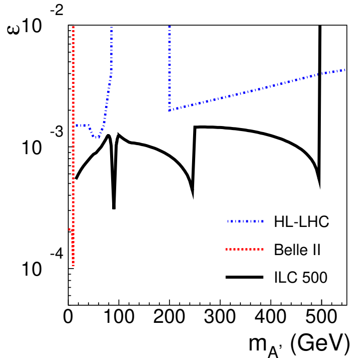
Figure 10.21: Projected reach of HL-LHC, Belle-II and the ILC for the dark Z gauge boson, in terms of its mass and the kinetic mixing parameter \varepsilon [616, 617].
