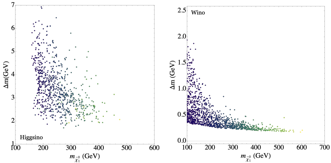
Figure 14.1: Scans over the parameter set of the MSSM giving models that account for the current discrepancy between the observed value of the muon g - 2 and the consensus SM prediction, from [676]. Left: Higgsino LSP; Right: Wino LSP. Other scenarios are described in the text. Color encodes the predicted value of the LSP dark matter density, with green indicating a higher value.
