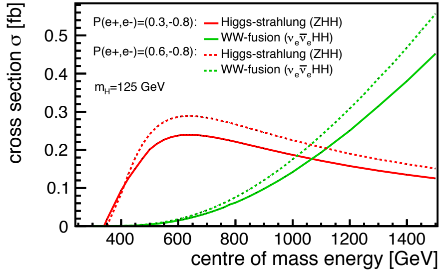
Figure 10.6: Cross-sections for double Higgs production in the SM via Higgs-strahlung and WW fusion as a function of the center-of-mass energy [511].
