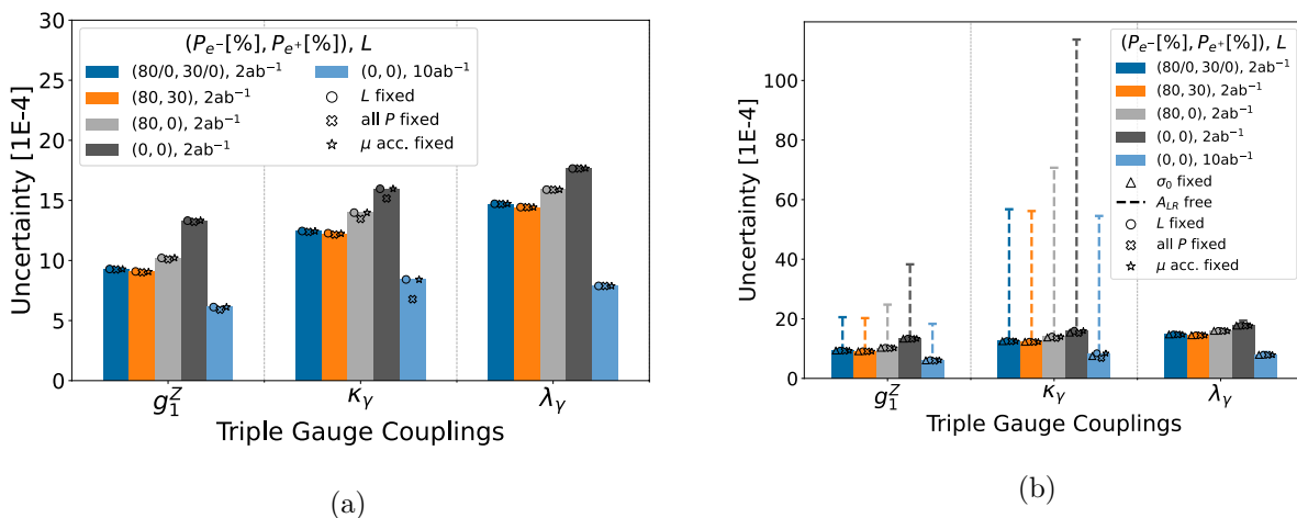
Figure 8.8: (a) Expected precisions at \sqrt{s} = 250 GeV of charged TGCs for different assumptions on the beam polarizations and the integrated luminosity. Note that these appear more pessimistic than in Fig. 10.9 since here only the \mu\nu q\bar{q} channel is used in a binned three-angle analysis (b) Effect of floating the left-right asymmetry of the the Zee coupling in the fit. This underlines, first, the importance of independently measuring this this quantity — not only on the Z pole, but at 250 GeV — and, second, the increased robustness of the fit due to beam polarization, which reduces the dependence on the left-right asymmetry considerably. Both from [380, 381].
