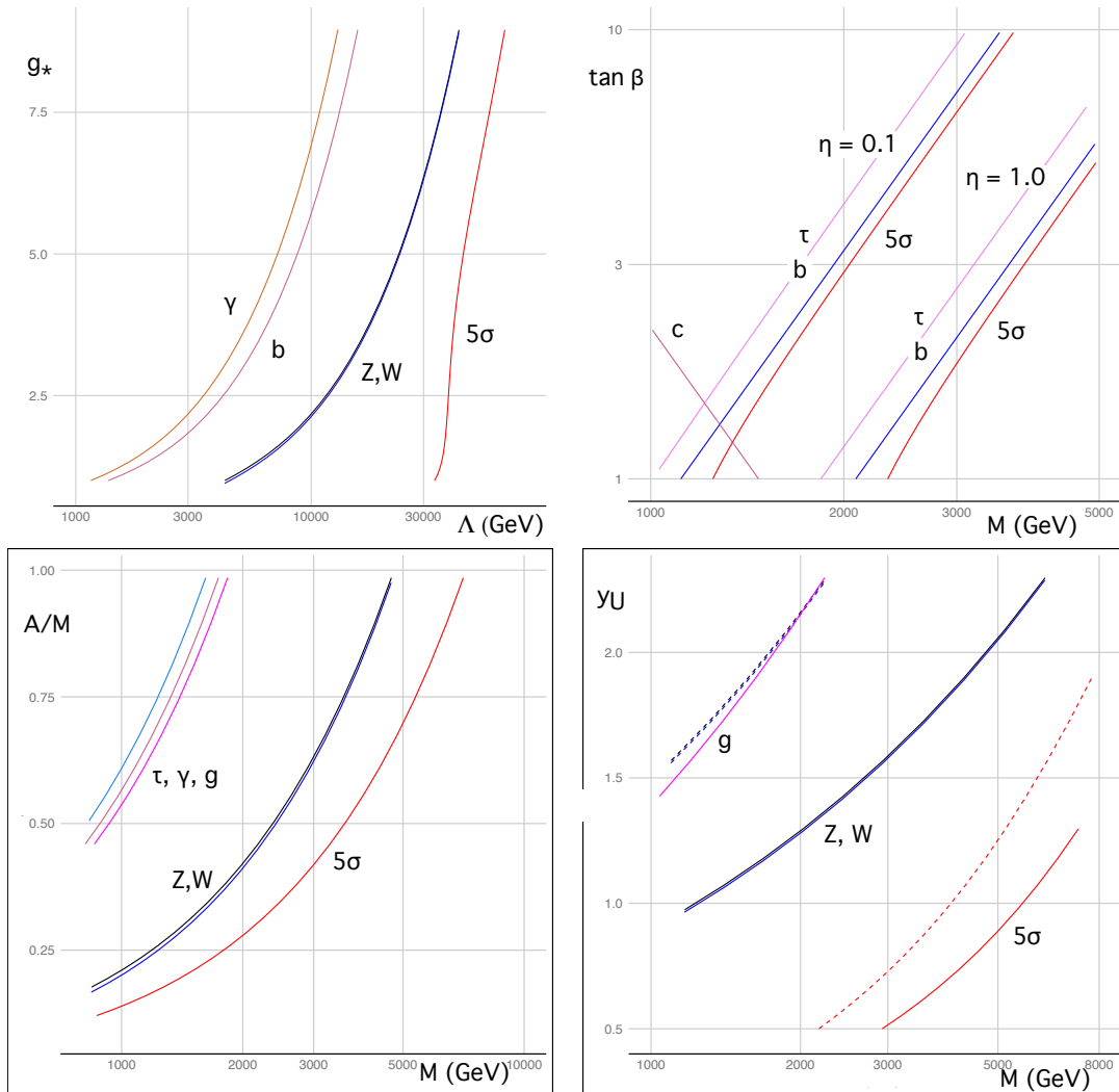
Figure 14.4: Mass reach of Higgs boson coupling deviations in a variety of scenarios reviewed in [707]. The curves give the 3\sigma sensitivity for particular Higgs boson couplings as a function of the new particle mass and a dimensionless parameter relevant to each scenario. The red curves on the right give the 5\sigma discovery contour for a fit of the full set of Higgs boson coupling measurements to ILC data. The scenarios are: (upper left) the Strongly Interacting Light Higgs, (upper right) two-Higgs doublet models, (lower left) models with a scalar singlet, (lower right) integration out of a vectorlike quark doublet.
