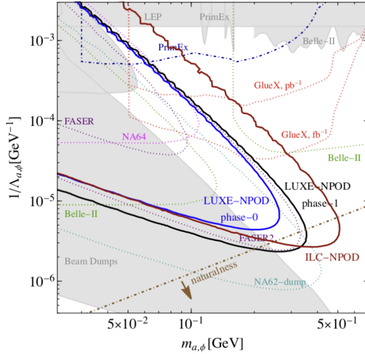
Figure 11.4: Sensitivity of the ILC version of the LUXE-NPOD experiment [631] searching for scalar and axion-like particles that couples to photons. The sensitivity is expressed in terms of parameters \Lambda_a and \Lambda_\phi defined in eq. (11.1).
