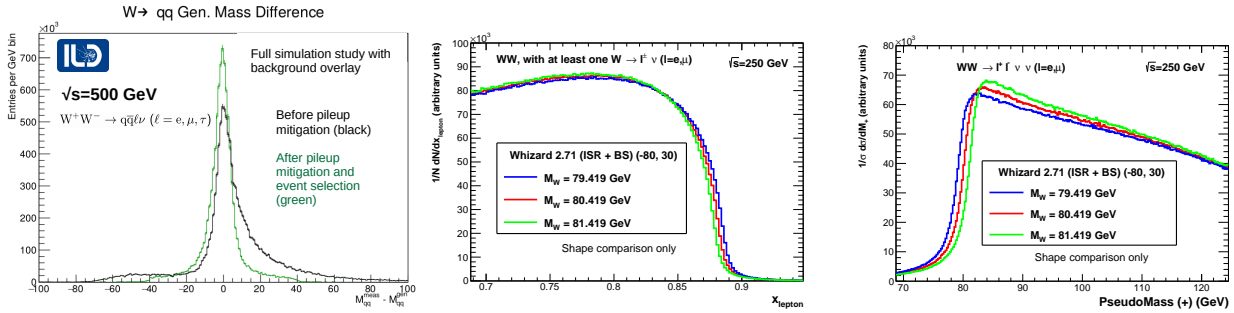
Figure 9.5: Illustrations of sensitivity to m_W . Hadronic mass resolution (left) in semi-leptonic events from full simulation study at \sqrt{s} = 500 GeV [448]. Endpoints and pseudomass methods at \sqrt{s} = 250 GeV (right).
