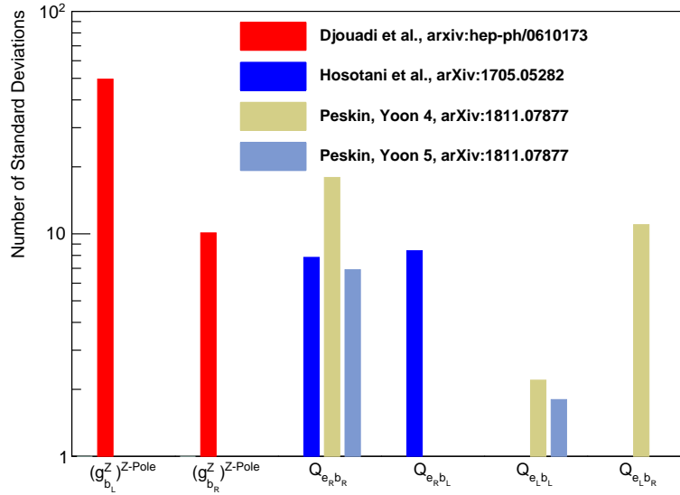
Figure 10.10: Visibility of deviations from the SM predictions in g_{b_j}^Z, g_{b_j}^Z (to do: still missing in this plot) and the helicity amplitudes Q_{e_i b_j} , in standard deviations, from combined ILC250/Z-Pole running, expected from new physics models with Randall-Sundrum extra dimensions [439, 535, 534].
