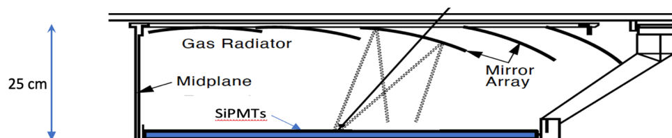
Figure 6.16: Proposed gaseous RICH detector addition to SiD/ILD [300].
