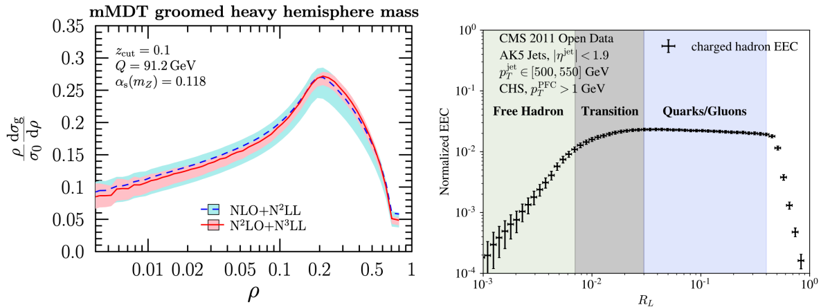
Figure 8.9: (a) The groomed mass observable in e^+e^- [388]. (b) A precision measurement of the two-point correlator in the collinear limit at the LHC [396]. Both of these new observables provide interesting probes of \alpha_s
