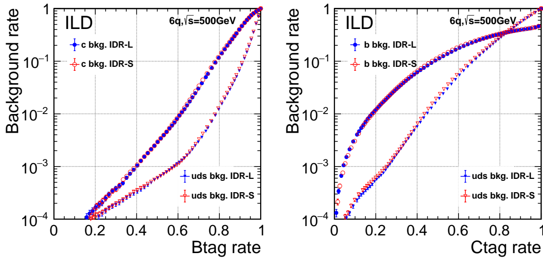
Figure 8.2: B-tag (left) and c-tag (right) performance in full-simulation studies of two variants of the ILD concept, IDR-L and IDR-S (figure from [214]).
