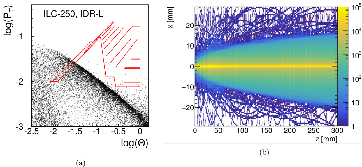
Figure 7.3: (a): Cones of incoherent e^+e^- -pairs in the ILD detector for E_{cms} = 250 \text{ GeV} as created with GuineaPig. Shown is \log p_t of the particles (radius of the helical trajectory) as a function of \log \theta . Also shown are the inner detector elements of the ILD detector (horizontal lines represent barrel elements and diagonal lines represent end-cap elements). (b): Cone of background from incoherent e^+e^- -pairs, generated with Guinea-Pig and simulated in the 5 T B-field of the SiD detector (from [326]).
