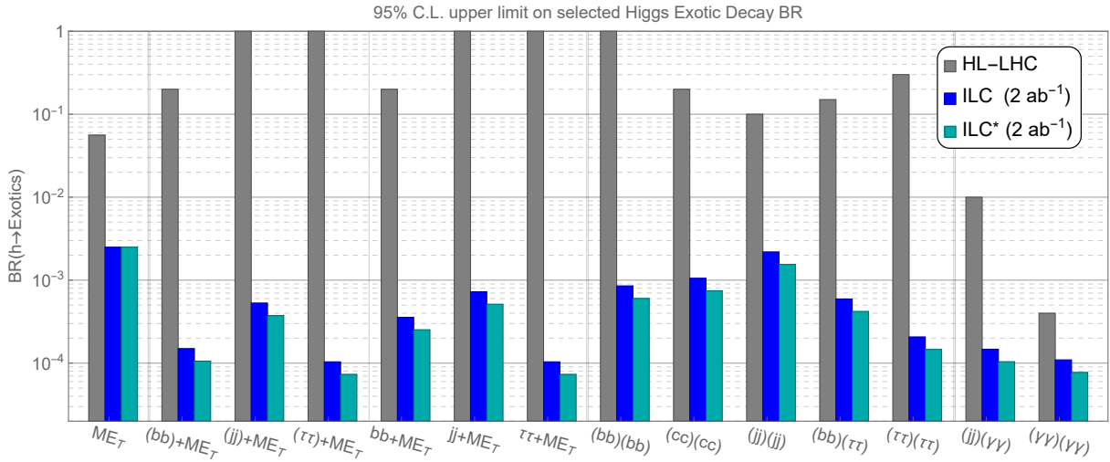
Figure 8.7: The 95% C.L. upper limit on selected Higgs exotic decay branching fractions at HL-LHC and ILC, based on Ref [346]. The ILC curves are derived using results from Ref [346] with leptonic decaying Z boson in the e^-e^+ \rightarrow ZH process. The ILC* scenario further utilizes the hadronically decaying Z boson and includes an estimated (indicative) improvement of 40%. Each set of three bars describes a different topology of exotic Higgs decay. For a recent review on current LHC constraints, see Ref. [348].
