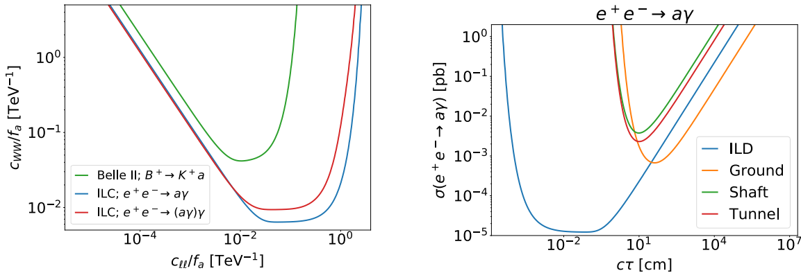
Figure 10.23: Left panel: Sensitivity projections for long-lived ALPs with m_a = 300 MeV at the ILC and at Belle II, as a function of the couplings c_{WW}/f_a and c_U/f_a . Right panel: Sensitivity projections for long-lived ALPs with m_a = 300 MeV at the ILC main detector (ILD), and three dedicated far-detector options (Ground, Shaft, and Tunnel). From Ref. [622].
