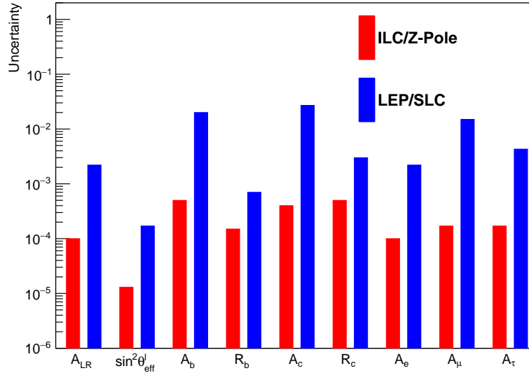
Figure 9.3: Summary of the precision achievable for ILC Z-Pole running compared with LEP/SLC results [426] for observables and derived quantities that are described in the text.
