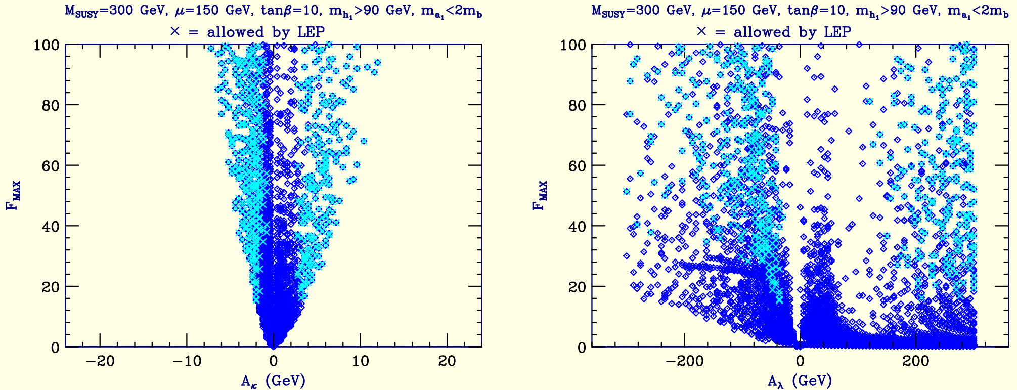
Figure 9: F_{\text{MAX}} vs. A_\kappa and A_\lambda for M_{\text{SUSY}} = 300 GeV, \tan \beta = 10 , \mu = 150 GeV after scanning over \lambda and \kappa values. All points have m_{a_1} < 2m_b . Light cyan \times points have large enough B(h_1 \rightarrow a_1 a_1) to escape LEP limits on Zh_1 \rightarrow Zb\bar{b} .
