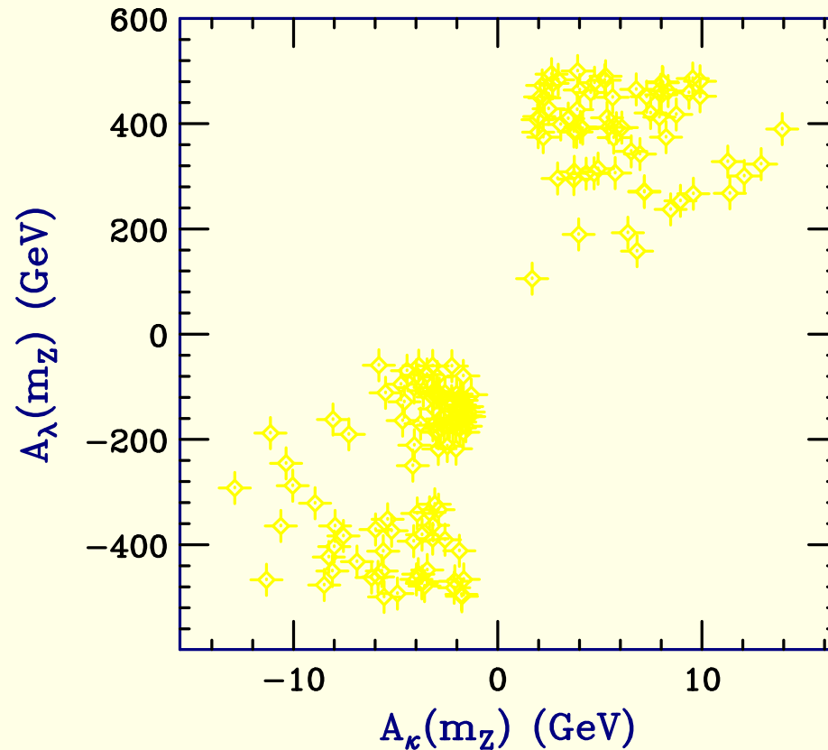
Figure 7: A_\kappa(m_Z) vs. A_\lambda(m_Z) for F < 25 fully ok m_{a_1} < 2m_b solutions in case of M_{1,2,3} = 100, 200, 300 GeV and \tan \beta = 10 . Note: A_\kappa, A_\lambda exactly 0 is not ok.
