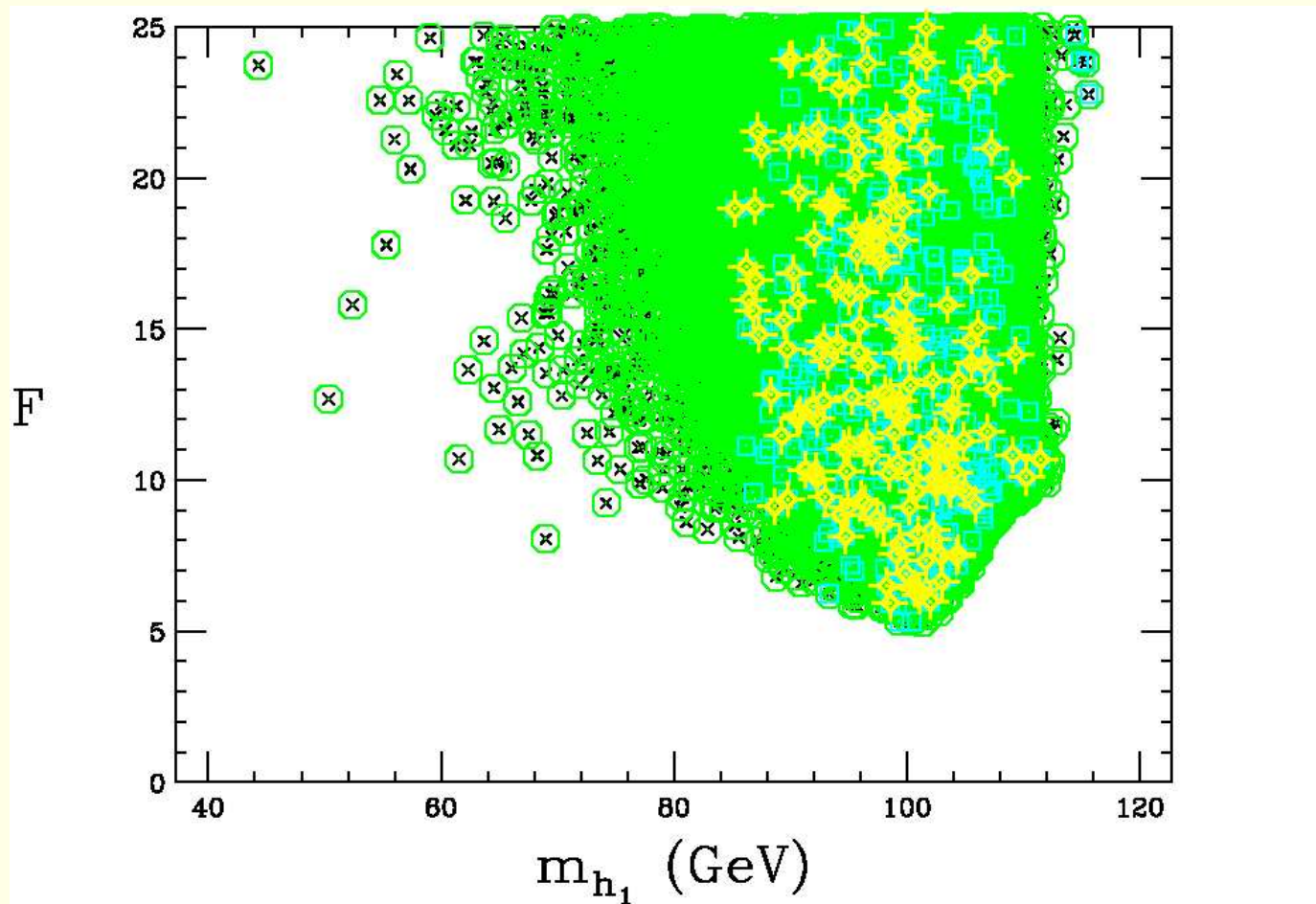
Figure 6: F vs. m_{h_1} for M_{1,2,3} = 100, 200, 300 GeV and \tan \beta = 10 . Small \times = no constraints other than global and local minimum, no Landau pole before M_U and neutralino LSP. The O 's = stop and chargino limits imposed, but NO Higgs limits. The \square 's = all single channel Higgs limits imposed. The large FANCY CROSSES are after requiring m_{a_1} < 2m_b .
