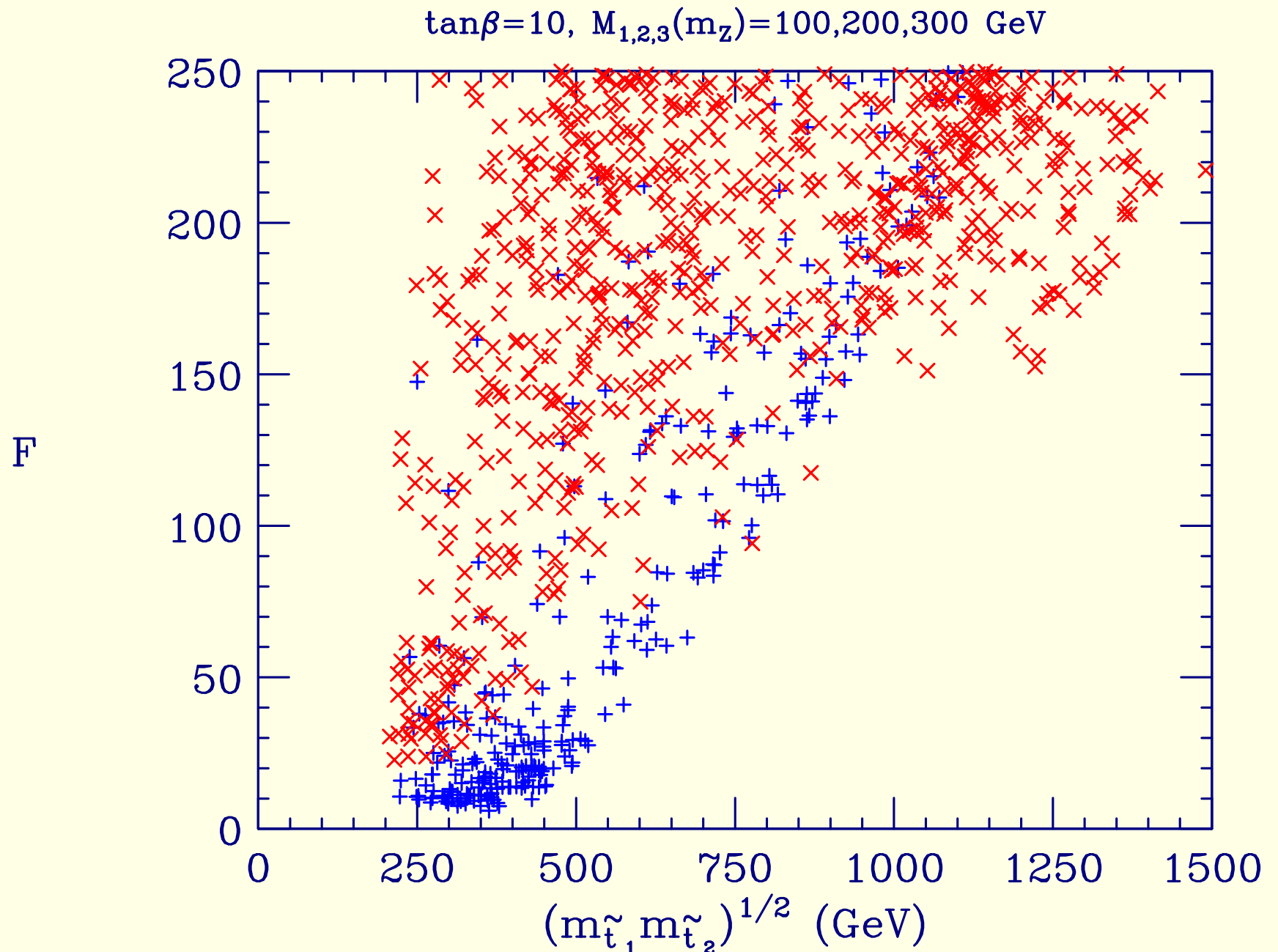
Figure 11: F as a function of root mean stop mass after latest single-channel LEP limits. Both m_{h_1} < 114 \text{ GeV} (+) and m_{h_1} \geq 114 \text{ GeV} (x) points are allowed.
